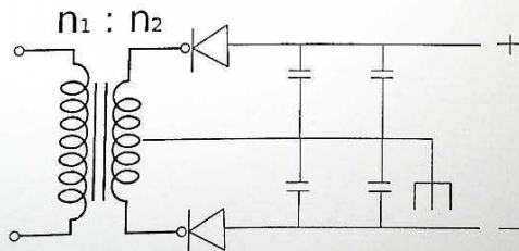
Fig. 4: capacitive filter
